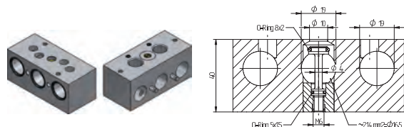
Individual valve isolation (R 5 104 K1 D1)
