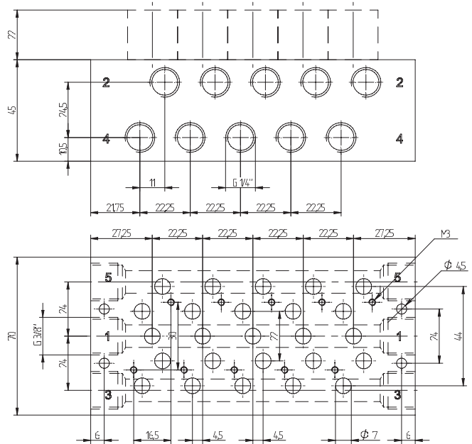
R 5__704 Orifice size: 10 mm
